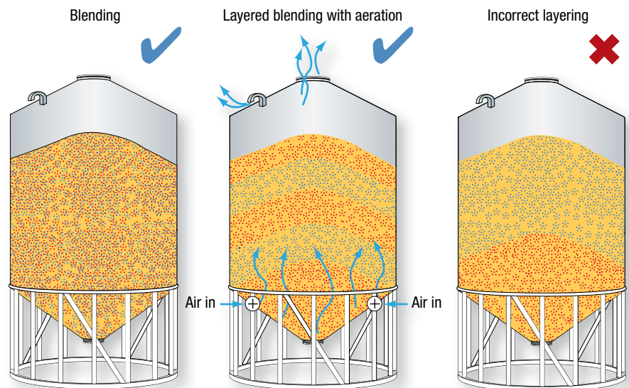
FIGURE 2 CORRECT BLENDING
